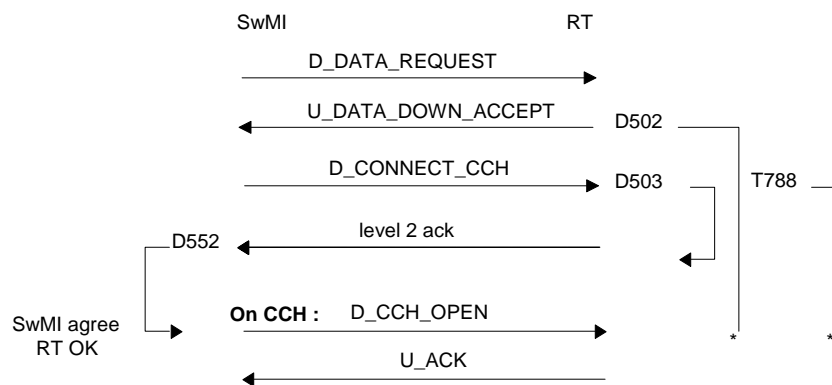
Figure 168: Downlink transmission request on CCH.
