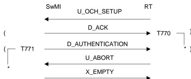
Figure 102: Open channel set-up failure RT side
