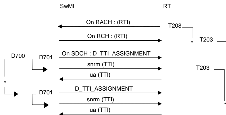
Figure 65: TTI negotiation sequence
