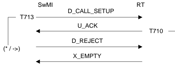
Figure 82: Incoming call failure SwMI side
