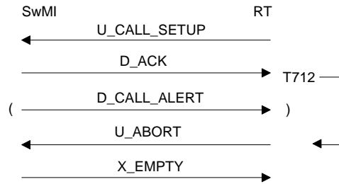
Figure 77: Outgoing call cancelled by the RT
