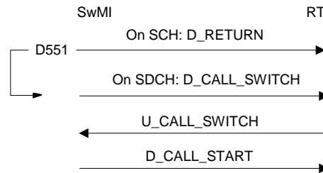
Figure 88: Transfer call sequence - calling RT side
