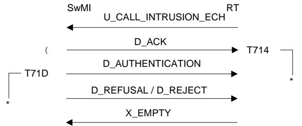
Figure 100: Emergency open channel intrusion failure SwMI side
