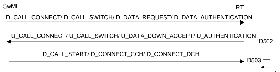
Figure 38: Connection to traffic channel sequence
