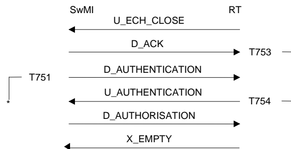
Figure 154: Emergency open channel release sequence
