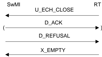
Figure 156: Emergency open channel release failure SwMI side
