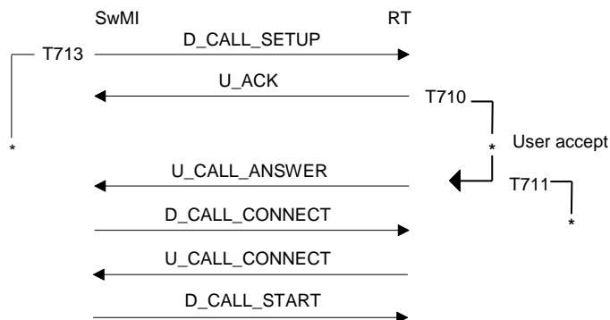
Figure 80: Incoming call sequence - case RT free
