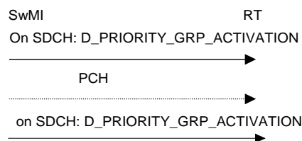
Figure 131: First D_ PRIORITY_GRP _ACTIVATION TSDU broadcast
