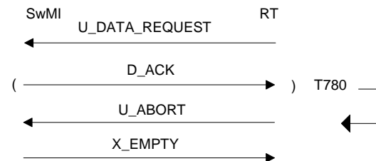
Figure 164: Failure in uplink transmission request (RT side)
