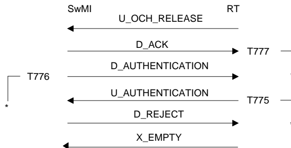
Figure 122: Open channel closing failure - authentication error
