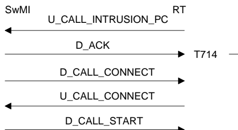
Figure 92: Private call intrusion sequence
