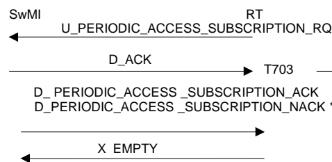
Figure 70: Periodic access subscription sequence
