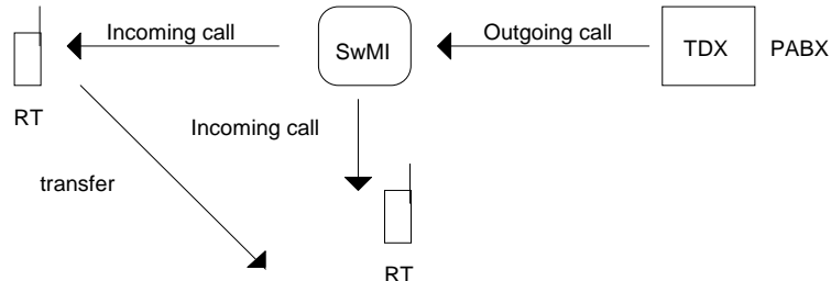
Figure 74: Incoming PABX Call with Call transfer
