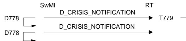
Figure 105: RT crisis notification at set-up
