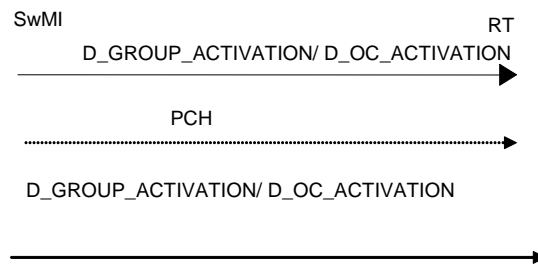
Figure 117: First D_XXX_ACTIVATION TSDU broadcast
