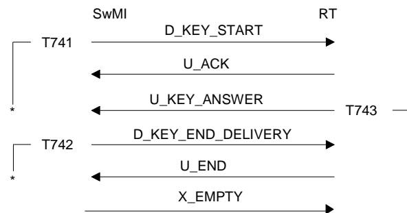
Figure 202: KEY delivery (with authentication)
