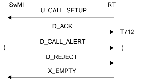
Figure 79: Outgoing call rejected by the SwMI
