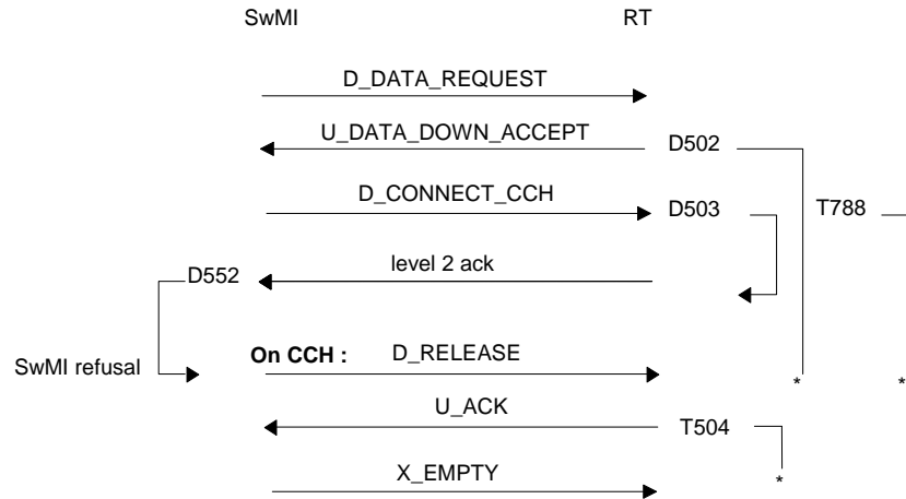
Figure 171: Failure in CCH downlink transmission request
