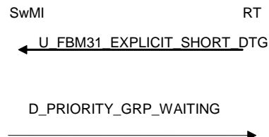
Figure 127: D_ PRIORITY_GRP _WAITING TSDU broadcast in FBM3.1 mode
