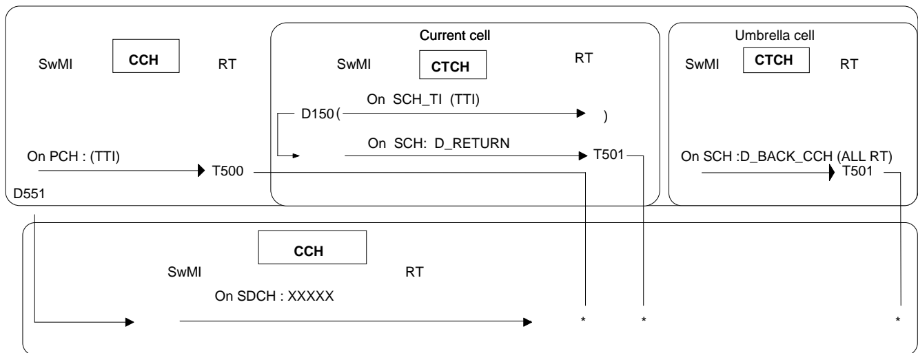
Figure 22: Paging - case RT free - immediate contact
