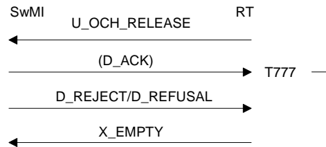
Figure 121: Open channel release failure SwMI side
