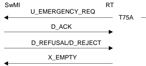
Figure 138: Emergency situation signalling failure SwMI side
