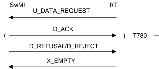
Figure 163: Failure in uplink transmission request (SwMI side).
