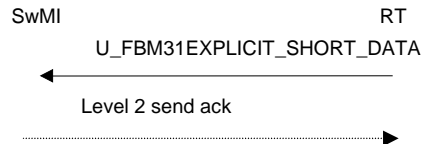
Figure 179: Short datagram transmission in FBM3.1 mode
