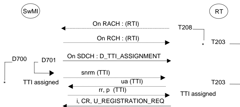
Figure 63: TTI negotiation sequence
