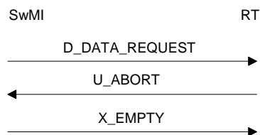
Figure 170: Failure in downlink transmission request (RT side)
