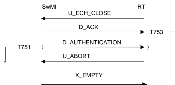
Figure 155: Emergency open channel release failure RT side
