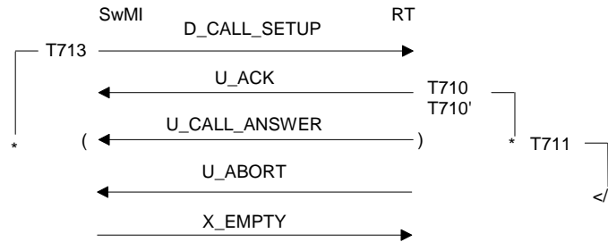
Figure 83: Incoming call failure RT side
