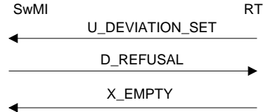
Figure 195: Start forwarding failure
