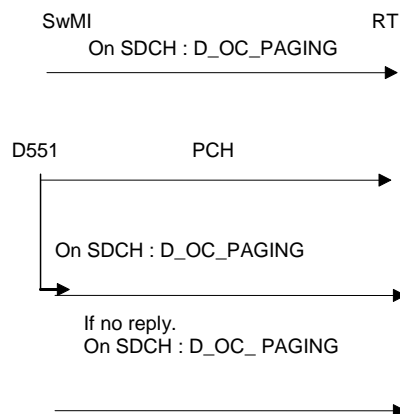
Figure 115: object call paging without RT answer
