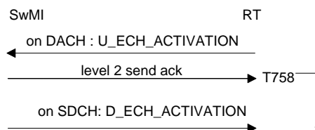
Figure 150: Emergency open channel activation request
