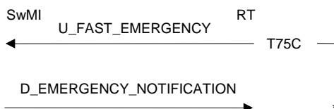
Figure 134: Emergency open channel signalling
