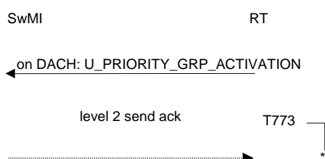
Figure 129: Tower communication Activation request failure on time-out
