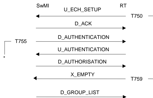
Figure 143: Emergency open channel set-up sequence
