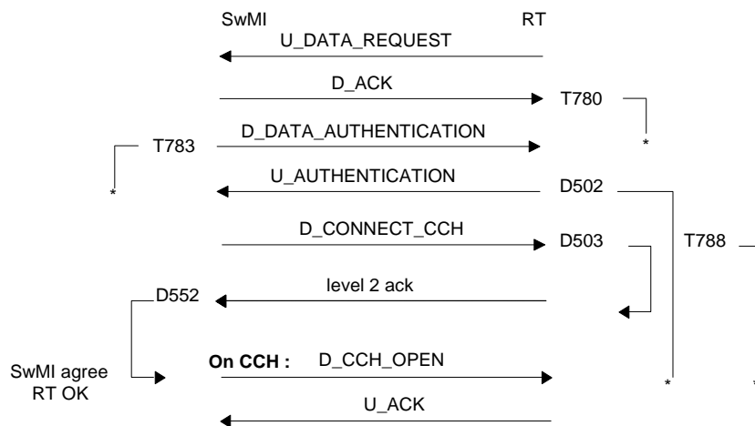
Figure 161: Uplink transmission request on CCH.
