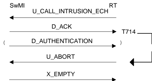
Figure 99: Emergency open channel intrusion failure RT side
