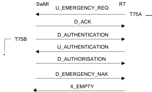
Figure 136: Emergency situation signalling (refused)
