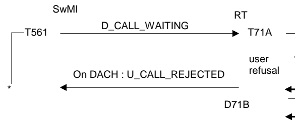
Figure 54: Private call or call from PABX, Call refused by one user
