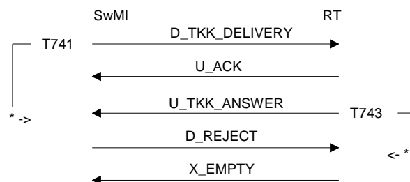
Figure 200: TKK delivery failure SwMI side
