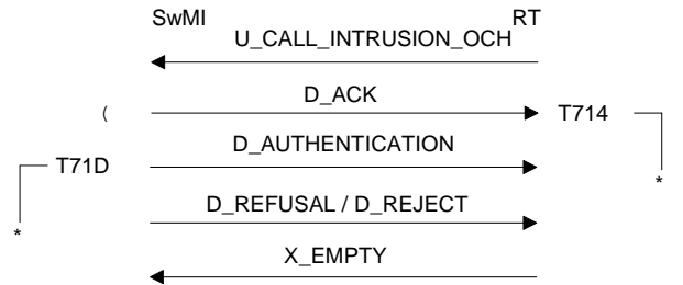
Figure 97: Open channel intrusion failure SwMI side
