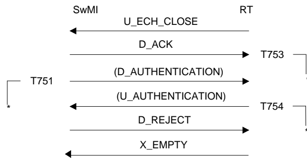
Figure 157: Emergency open channel release failure - authentication error
