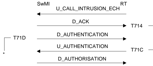
Figure 98: Emergency open channel intrusion sequence
