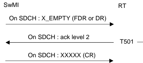
Figure 19: Paging - case RT engaged in an application transaction
