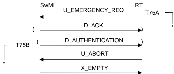
Figure 137: Emergency situation signalling failure RT side
