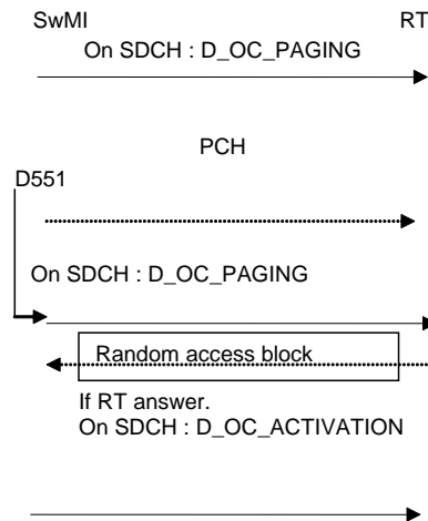
Figure 114: object call paging with RT answer
