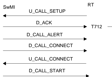
Figure 76: Outgoing call sequence
