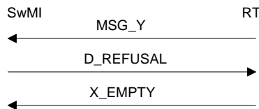
Figure 27: Paging failure SwMI side - error in TSDU
