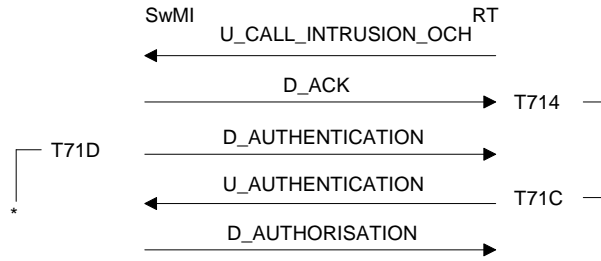
Figure 95: Open channel intrusion
