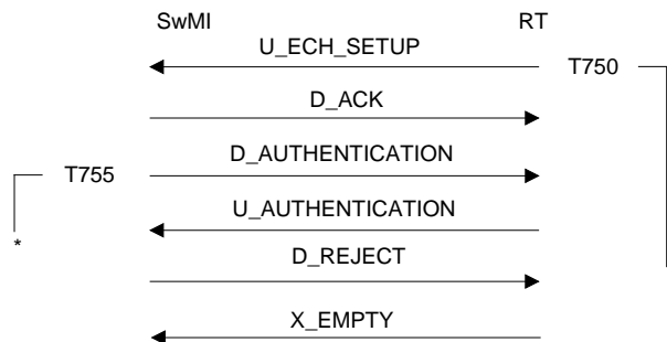
Figure 146: Emergency open channel set-up failure - authentication error
