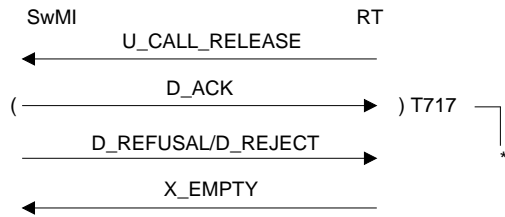
Figure 90: Release call request refused by the SwMI
