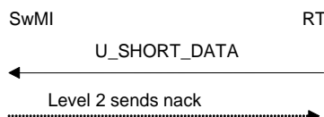
Figure 177: Short datagram transmission failure
