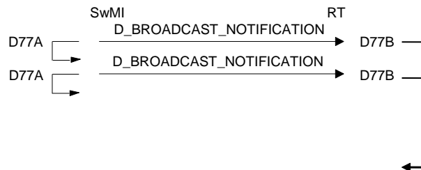
Figure 106: RT broadcast notification at set-up
