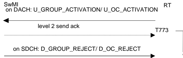
Figure 111: Activation request reject
