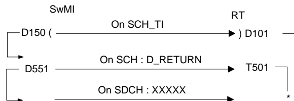
Figure 20: Paging - case RT accessible - immediate contact
