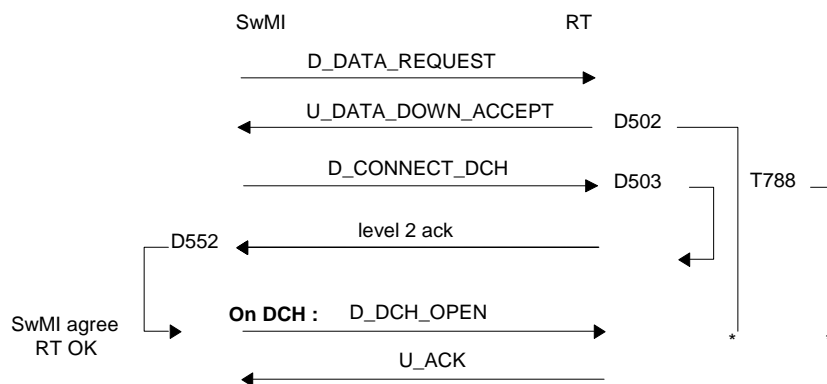
Figure 169: Downlink transmission request on DCH.
