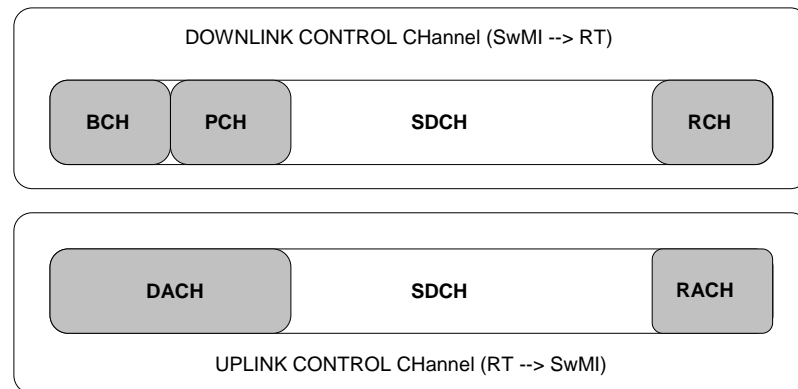
Figure 2: Main Control channel model
