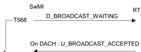
Figure 57: Broadcast message accepted by one user
