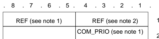
Figure 14: 2 header octets in the first application transaction TSDU
