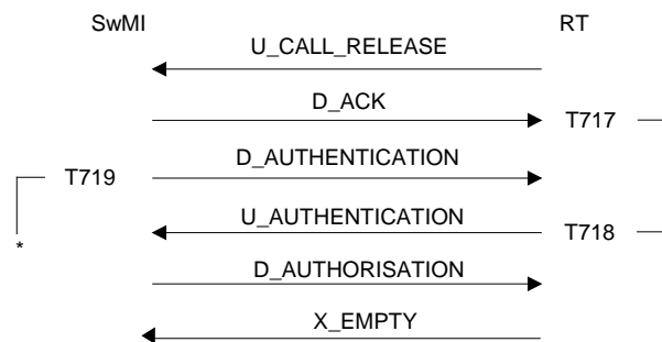
Figure 89: Release call request sequence
