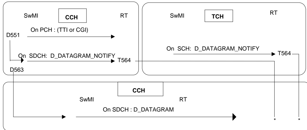
Figure 183: Asynchronous broadcast sequence
