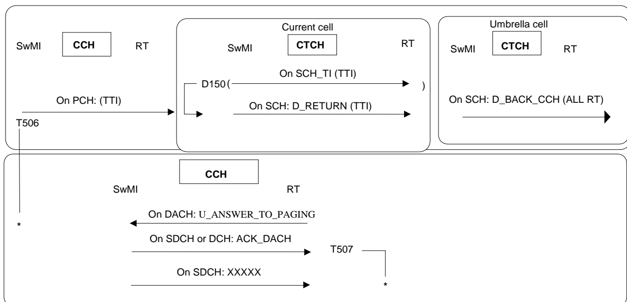
Figure 23: Paging - case RT free - acknowledged contact
