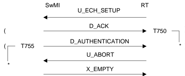
Figure 144: Emergency open channel set-up failure RT side
