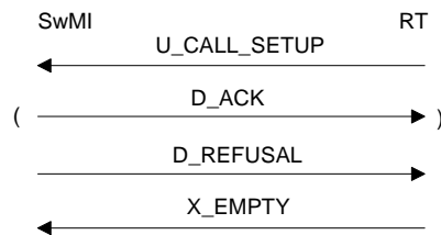
Figure 78: Outgoing call refused by the SwMI
