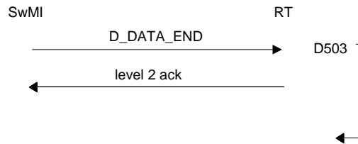
Figure 175: End of the transmission
