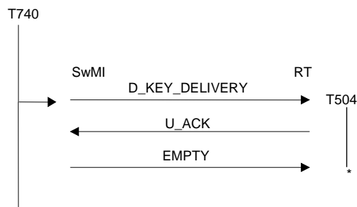
Figure 201: KEY delivery sequence with no segmentation
