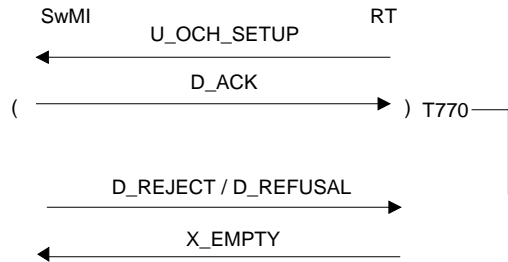
Figure 103: Open channel set-up failure SwMI side
