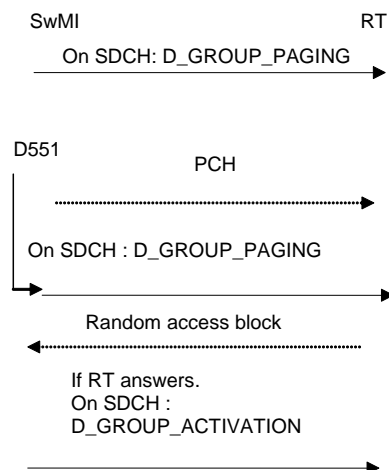
Figure 112: paging with answer from RT
