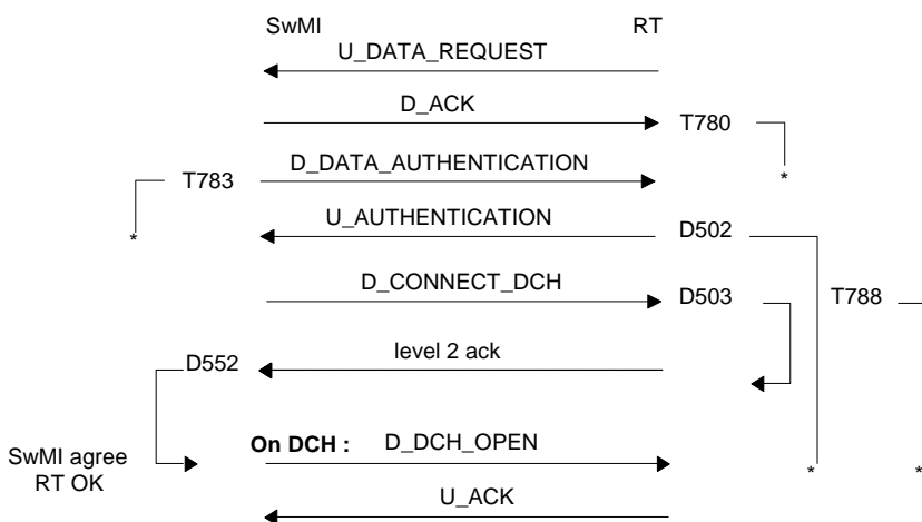
Figure 162: Uplink transmission request on DCH.
