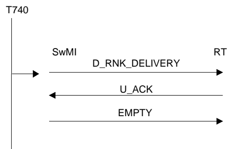
Figure 198: RNK delivery sequence
