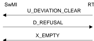
Figure 197: Stop forwarding failure
