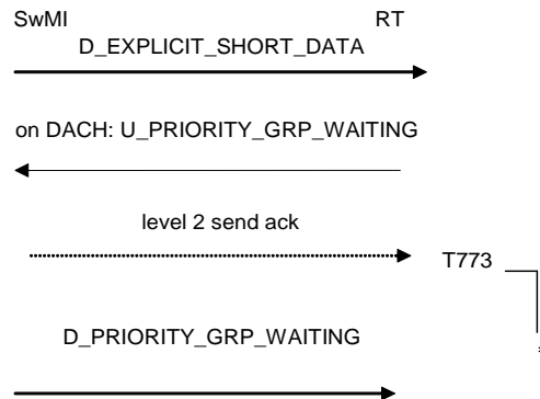
Figure 125: tower communication speech request acknowledgement
