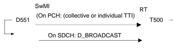
Figure 182: General Broadcast sequence
