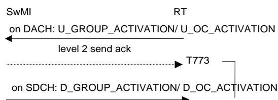
Figure 108: Group communication Activation
