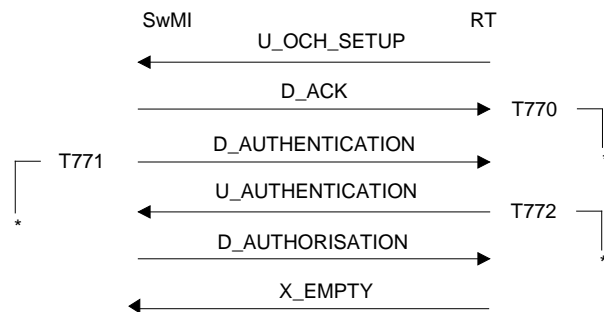
Figure 101: Open channel set-up sequence
