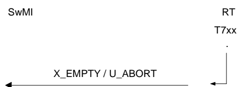
Figure 30: Application transaction failure
