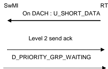
Figure 126: D_ PRIORITY_GRP _WAITING TSDU broadcast in nominal mode
