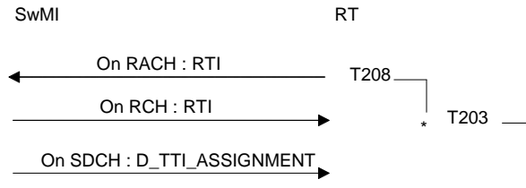
Figure 64: TTI negotiation - Unsuccessful case
