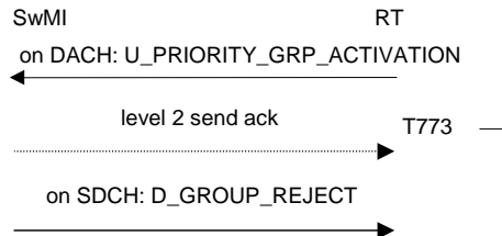
Figure 130: Tower communication Activation request reject
