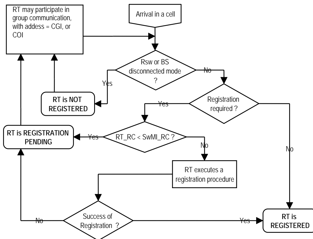
Figure 62: RT registration states
