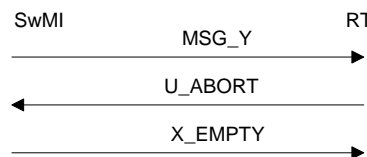
Figure 25: Dialogue failure RT side - error in TSDU
