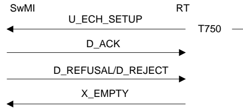
Figure 145: Emergency open channel set-up failure SwMI side
