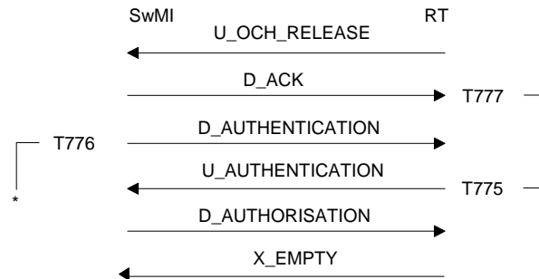
Figure 119: Open channel release sequence
