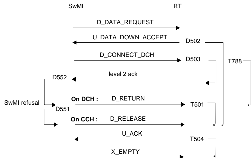
Figure 172: Failure in DCH downlink transmission request
