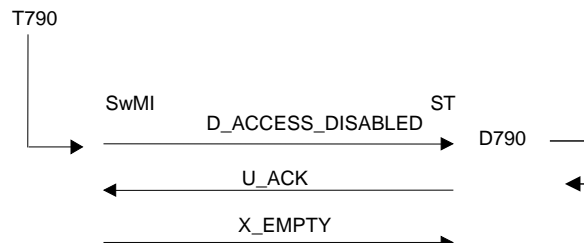
Figure 187: RT access disabling
