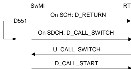
Figure 81: Incoming call sequence - case RT accessible
