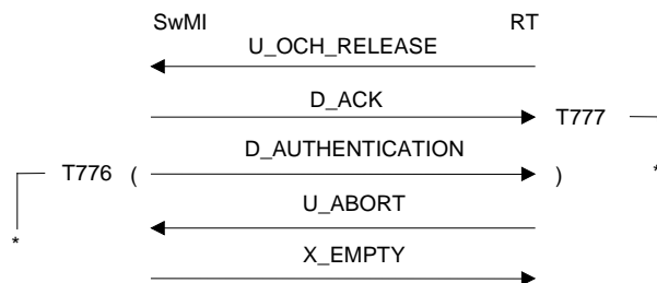
Figure 120: Open channel closing failure RT side
