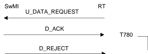
Figure 165: Failure in uplink transmission request (RT side)
