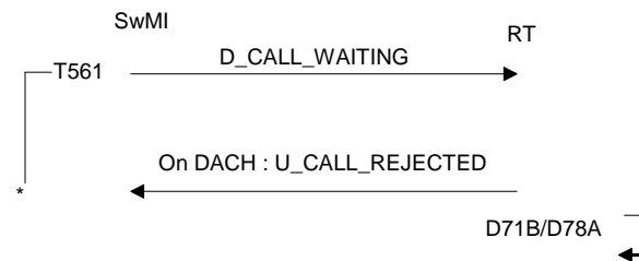
Figure 55: Data call or incoming PABX Call refusal by one RT
