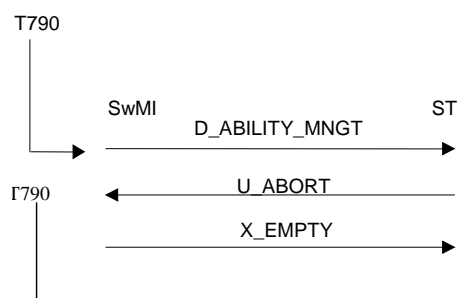
Figure 190: Unsuccessful case of enhanced protocol
