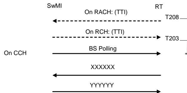
Figure 18: RACH / RCH transmission
