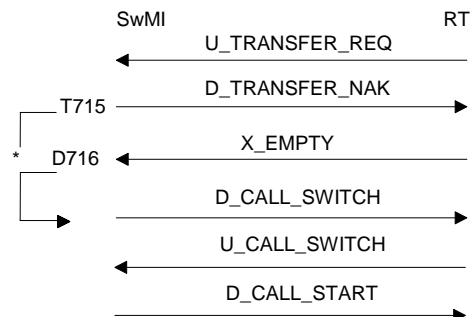
Figure 87: Call transfer request failure SwMI side
