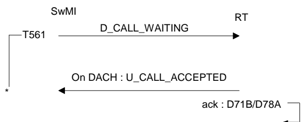
Figure 53: Data call or call for TDX accepted by one RT
