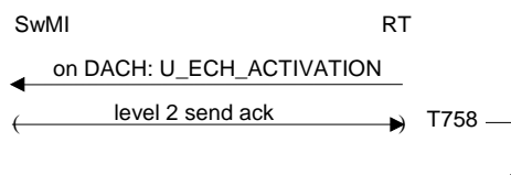
Figure 151: Emergency open channel activation request failure
