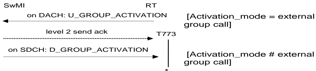
Figure 110: Group communication Activation failure (external group call)
