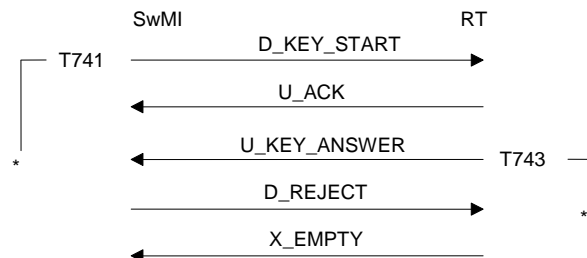
Figure 203: KEY delivery (with authentication) failure SwMI side
