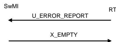
Figure 51: Fault reporting sequence
