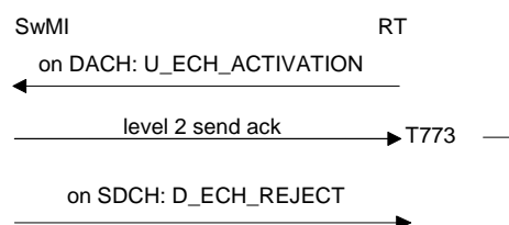
Figure 152: Activation request reject
