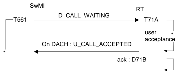
Figure 52: Private call accepted by one user
