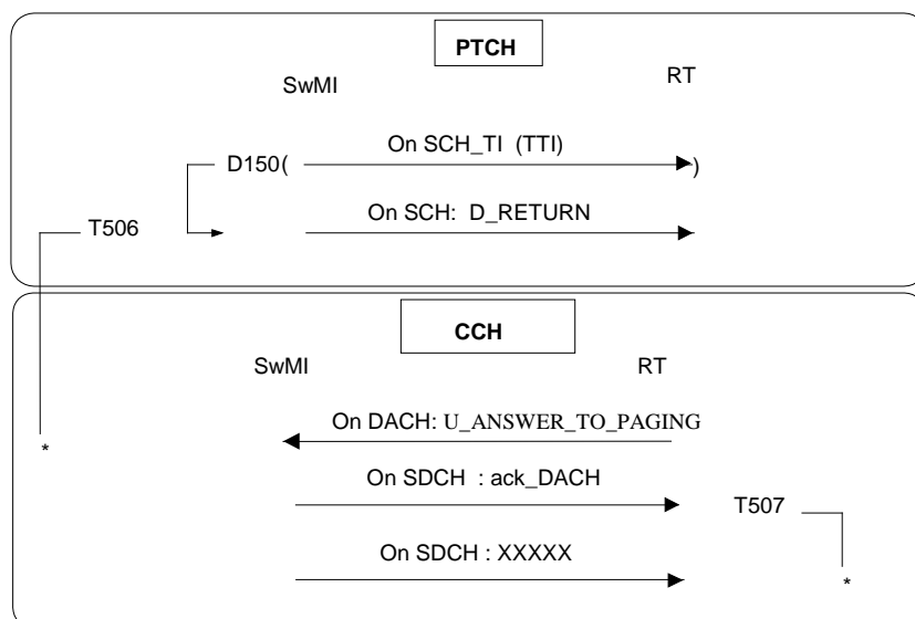
Figure 21: Paging - case RT accessible - acknowledged contact
