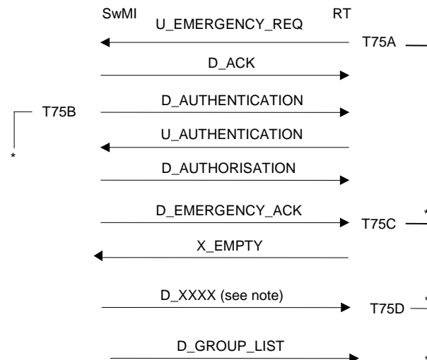
Figure 135: Emergency situation signalling (accepted)
