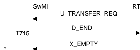
Figure 86: Call transfer request sequence
