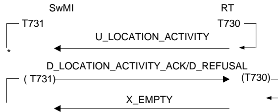
Figure 68: Location Activity transaction
