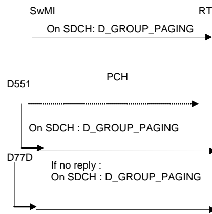
Figure 113: paging with no answer from RT
