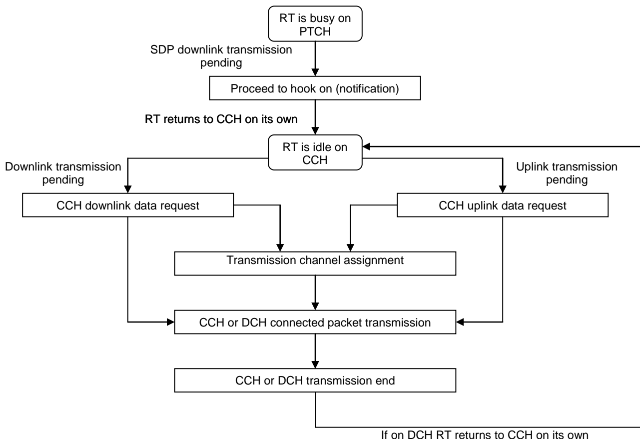
Figure 159: Connected packet transmission states
