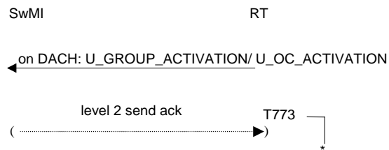
Figure 109: Activation request failure on time-out
