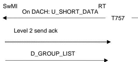
Figure 133: Emergency open channel signalling
