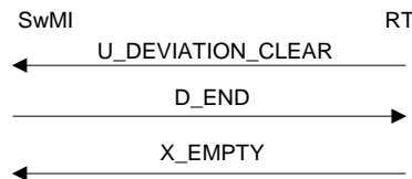
Figure 196: Stop forwarding sequence
