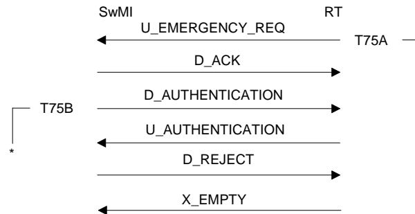
Figure 139: Emergency situation signalling failure - authentication error
