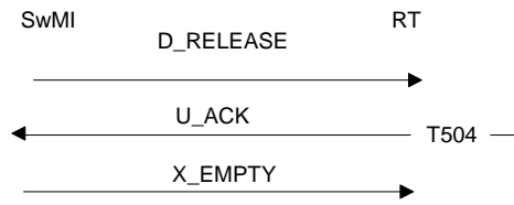
Figure 84: Private call release indication
