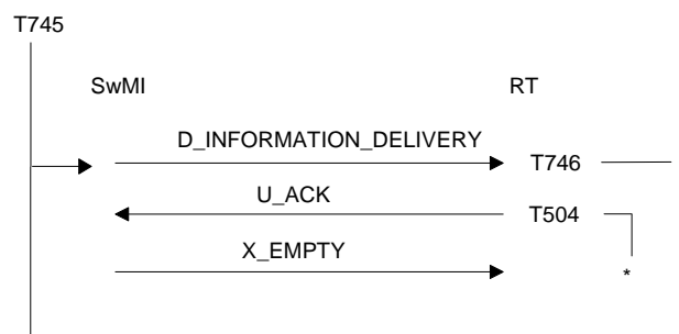
Figure 204: Information delivery sequence
