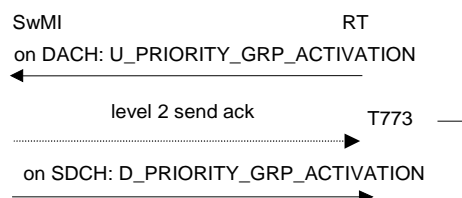
Figure 128: tower communication Activation from AG
