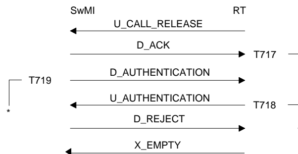
Figure 91: Release call request - RT authentication failure
