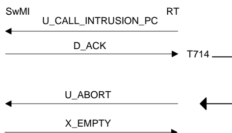
Figure 93: Private call intrusion failure RT side
