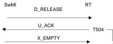
Figure 35: Application transaction release by the SwMI
