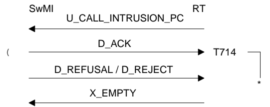
Figure 94: Private call intrusion failure SwMI side
