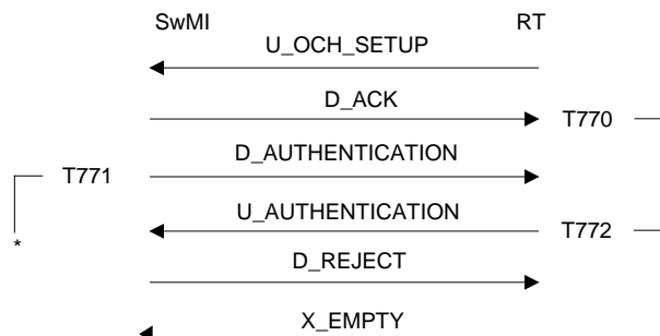
Figure 104: Open channel set-up failure - RT authentication error
