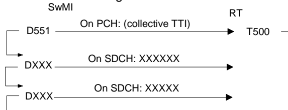
Figure 37: Asynchronous broadcast sequence
