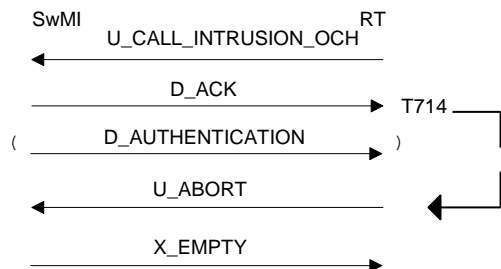
Figure 96: Open channel intrusion sequence
